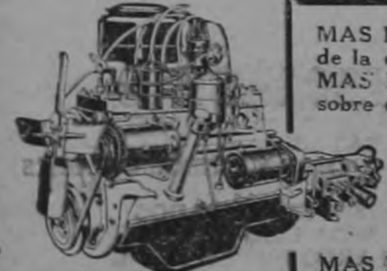
Motor SUPER. HURACAN WILLYS 115 H.P.
